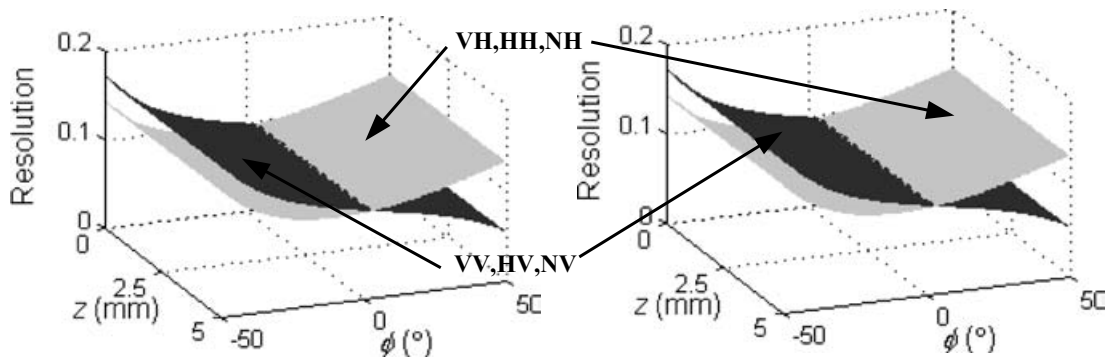
Fig. 19. Distributions of the y & z directional resolutions by the unit movement of the Z_{f1} fine actuator.
