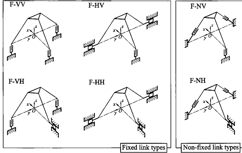
Fig. 15. Six possible architectures with fine actuators.
