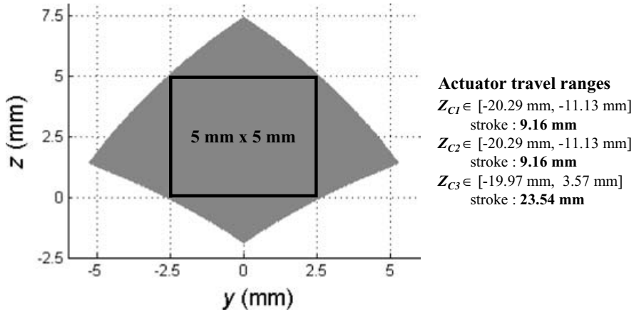
Fig. 11. Workspace of the miniaturized micro parallel mechanism.
