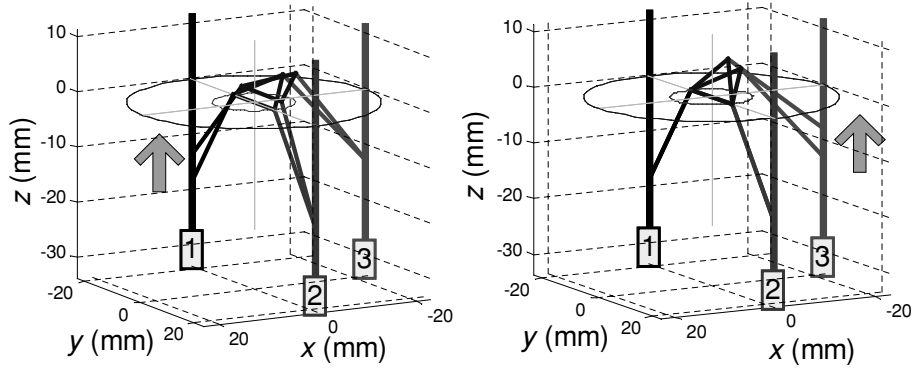
(a) Unit movement of the Z_{f1} actuator ( y, z )
