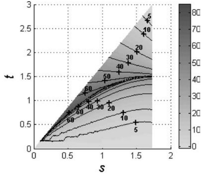
Fig. 4. Middle angle \phi_m ( ^\circ ) distribution within the PMSS.
