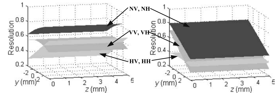
Fig. 18. Evaluation method for the platform resolution (VV type fine actuator architecture).
